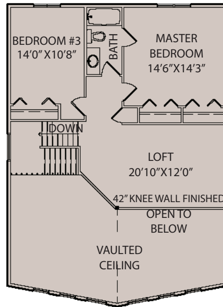
2ND FLOOR
